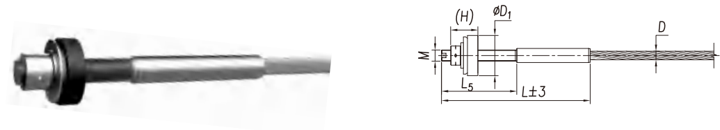
Adjustable End of Spherical Hinge C01
