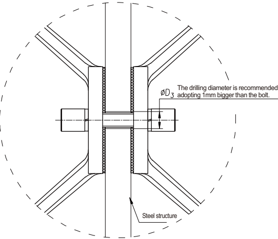
The clamping type of steel structure
