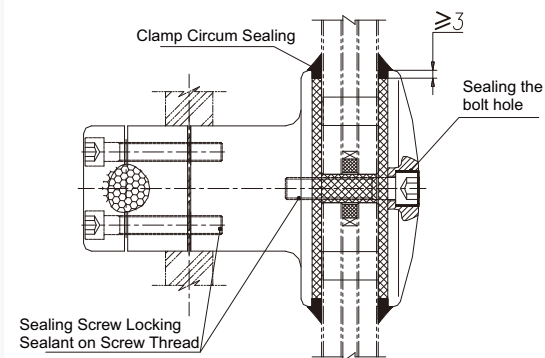
Picture One Water Proof & Anti-loose Illustrate Diagram
