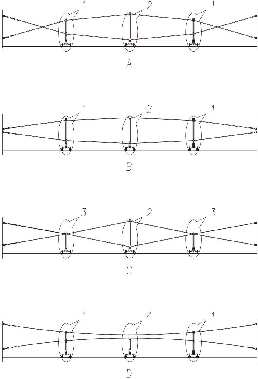
Forms of Horizontal Cable Arrangement
