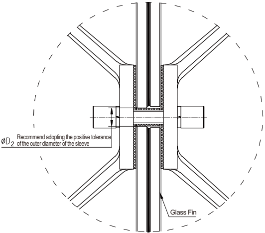
The clamping type of glass fin
