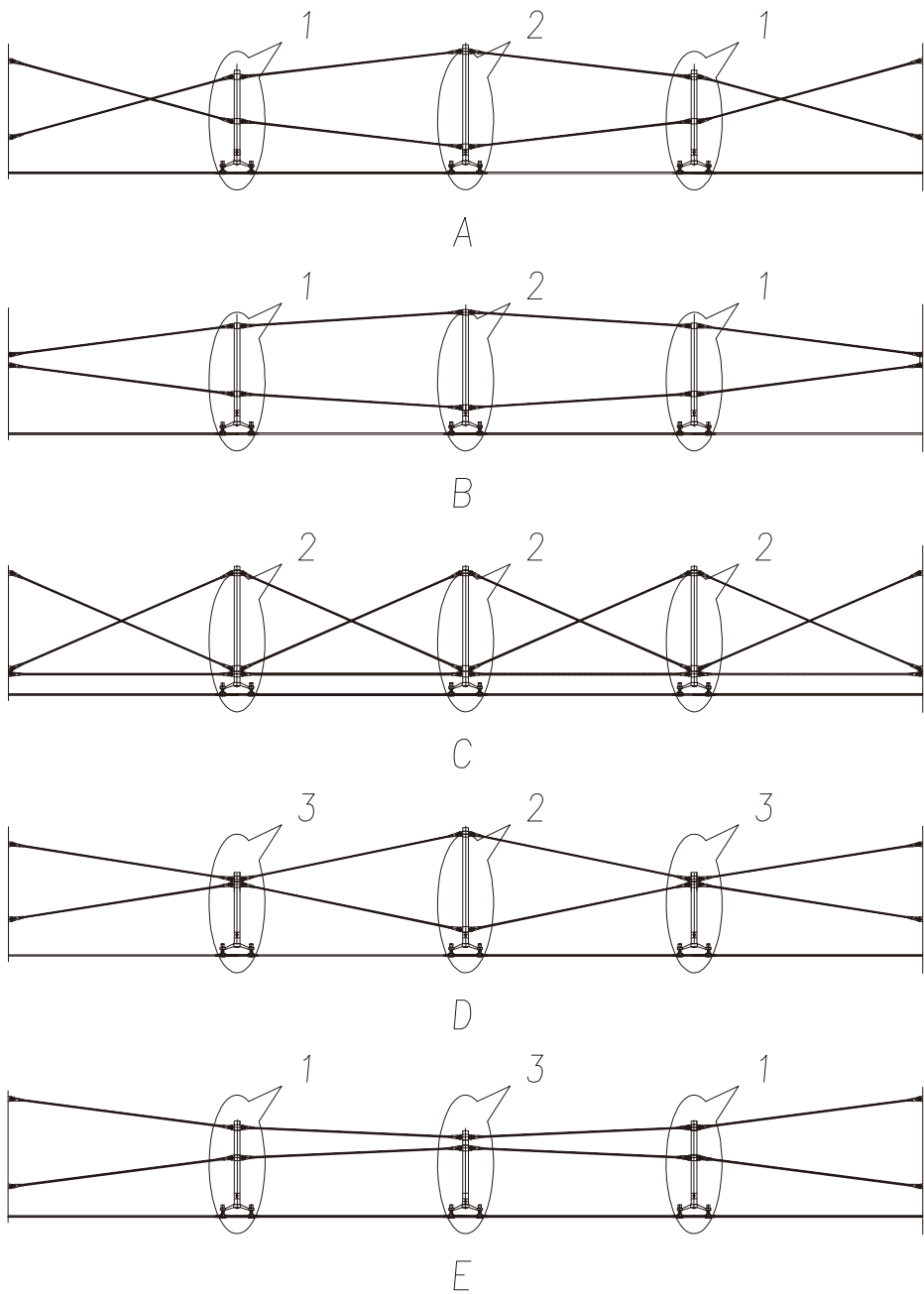
Forms of Horizontal Rod Arrangement
